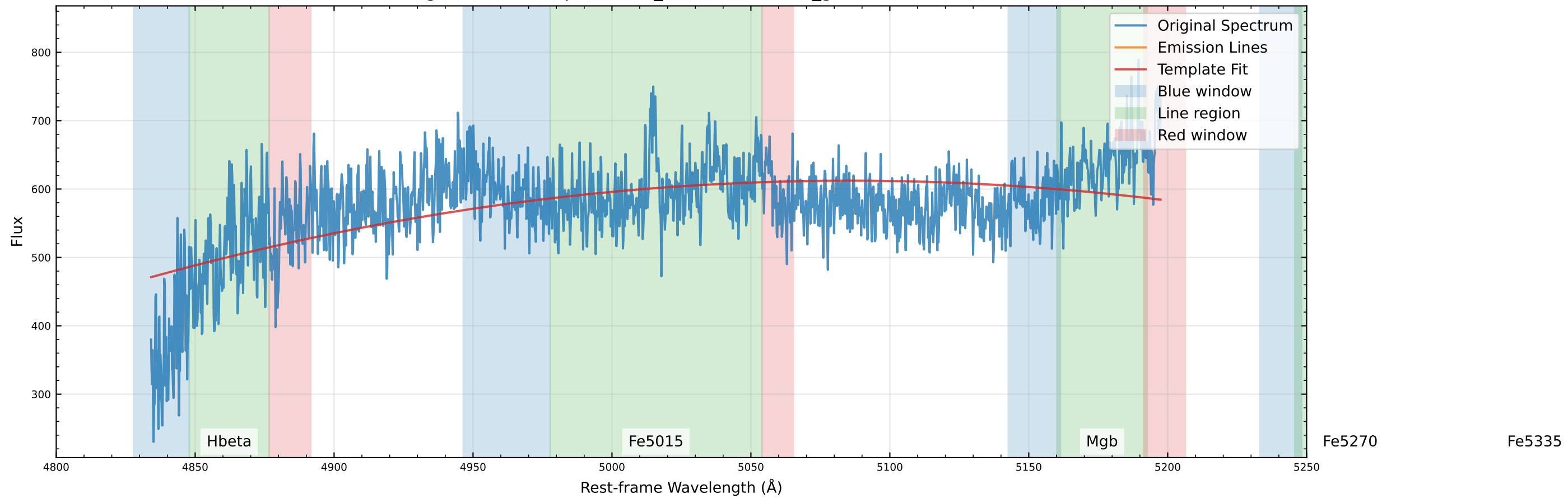
Original Data Comparison (v_star=0.0 km/s, v_gas=82.5 km/s)
