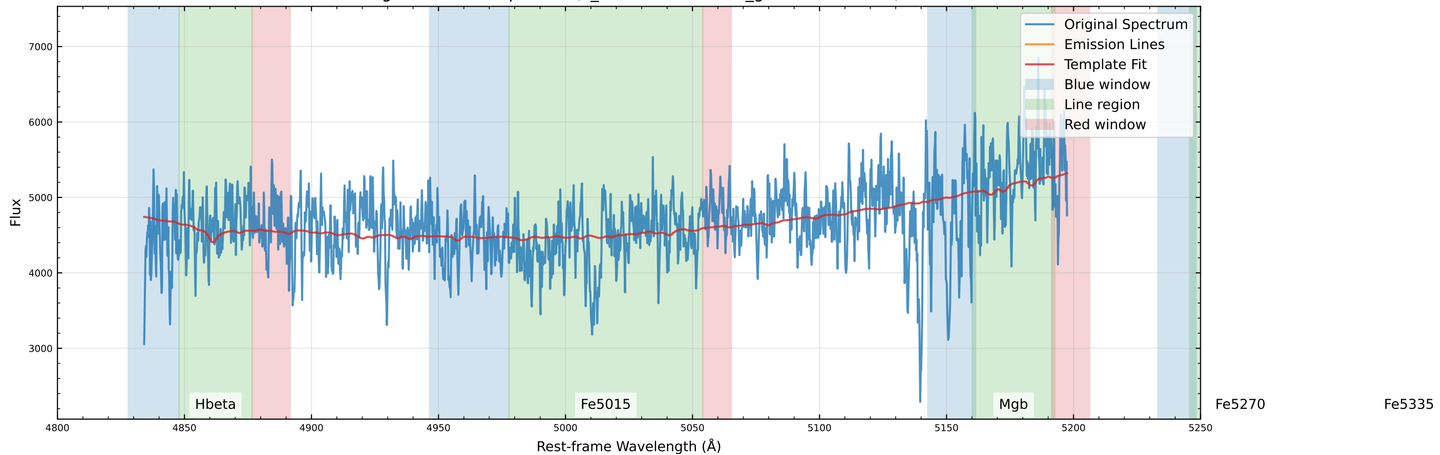
Original Data Comparison (v_star=42.2 km/s, v_gas=-249.5 km/s)
