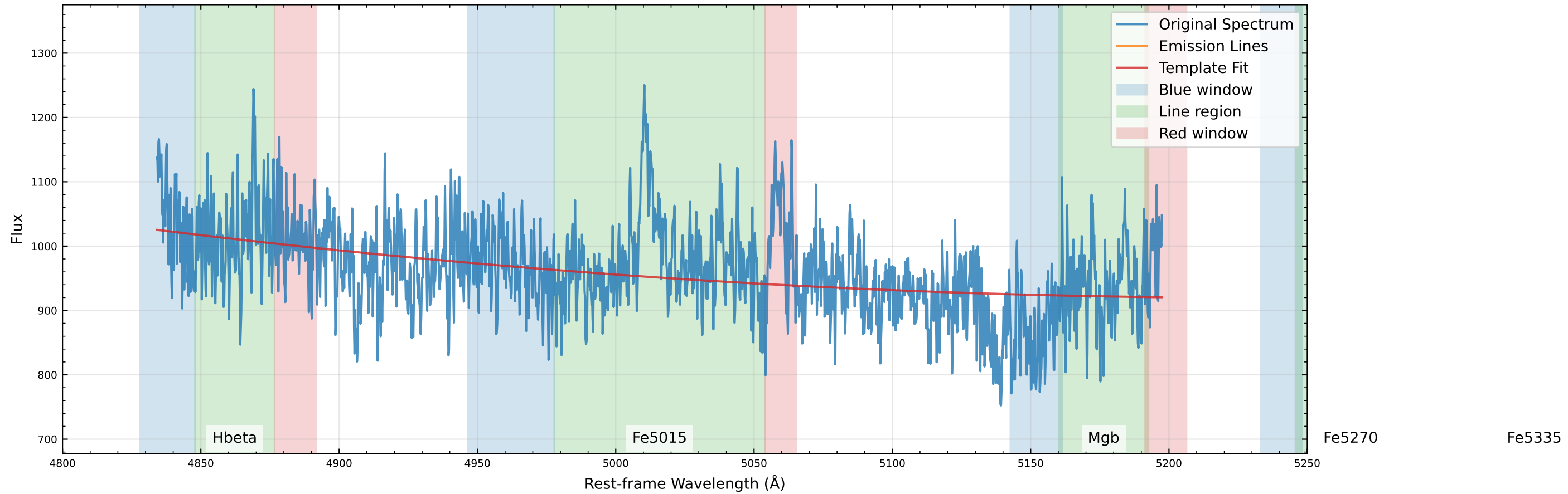
Original Data Comparison (v_star=0.0 km/s, v_gas=282.3 km/s)
