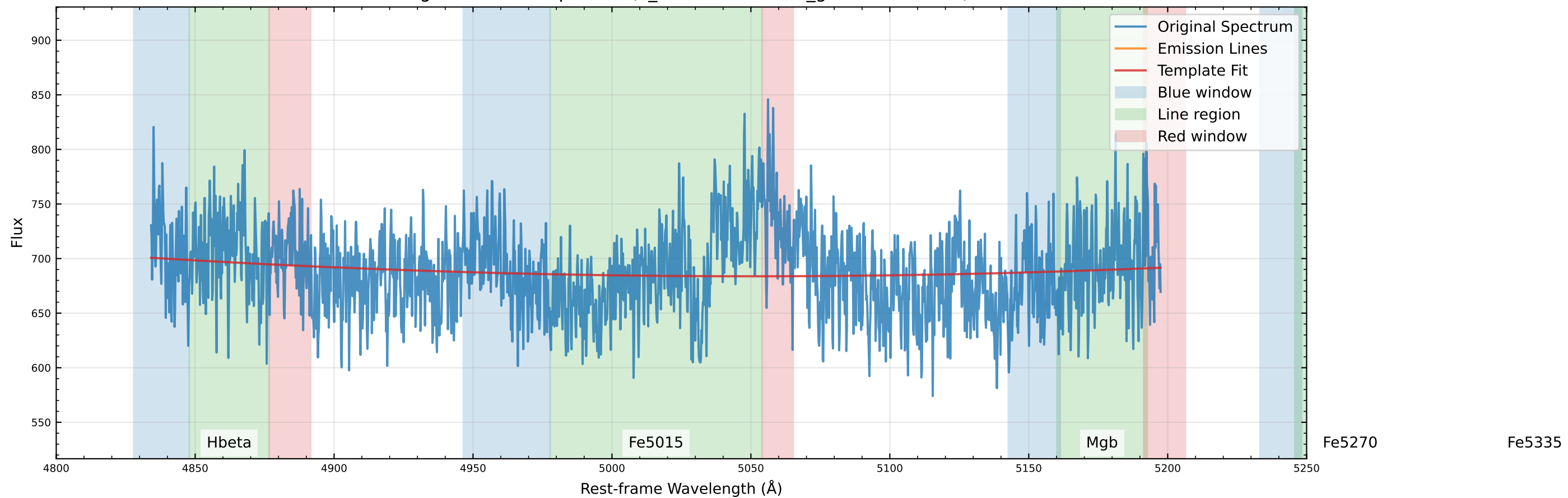
Original Data Comparison (v_star=0.0 km/s, v_gas=281.1 km/s)
