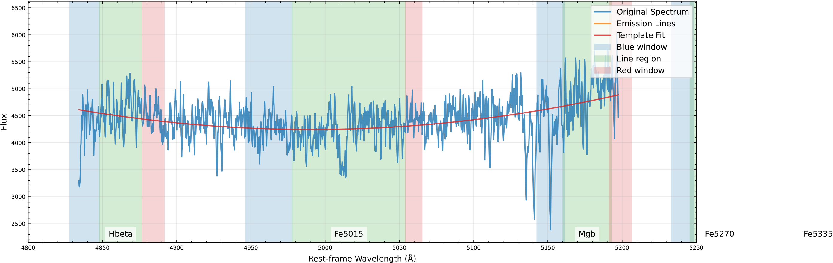
Original Data Comparison (v_star=0.0 km/s, v_gas=-9.7 km/s)
