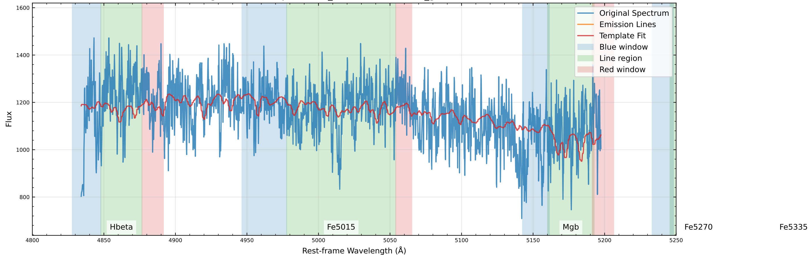
Original Data Comparison (v_star=-512.1 km/s, v_gas=-411.5 km/s)
