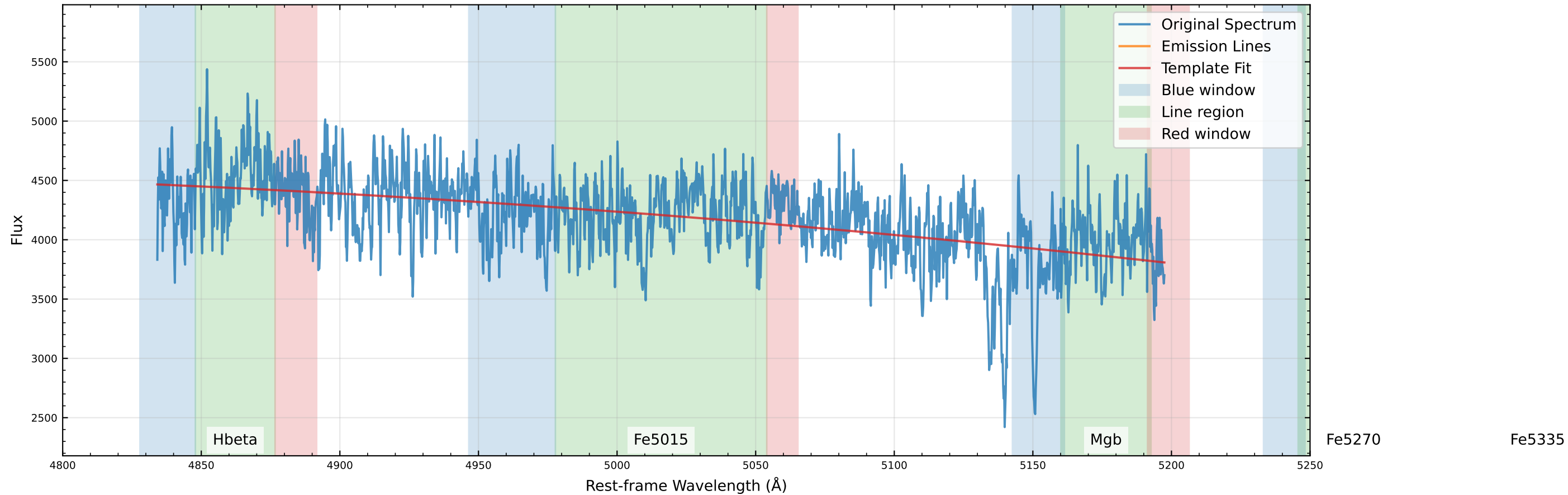
Original Data Comparison (v_star=0.0 km/s, v_gas=77.5 km/s)
