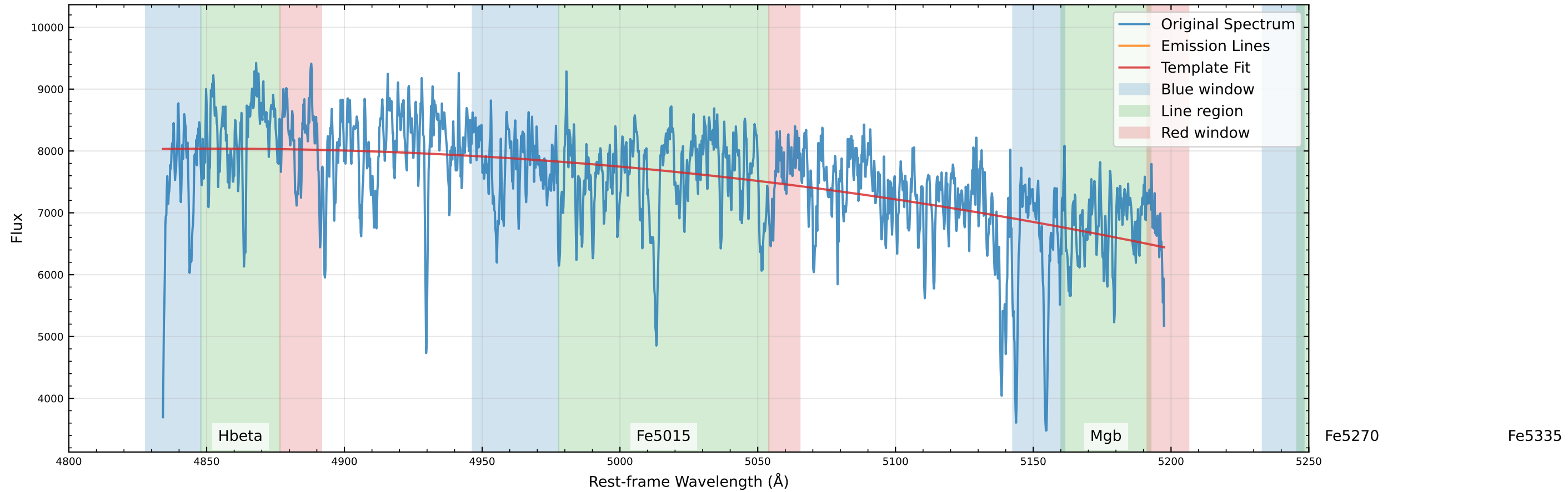
Original Data Comparison (v_star=0.0 km/s, v_gas=-64.7 km/s)
