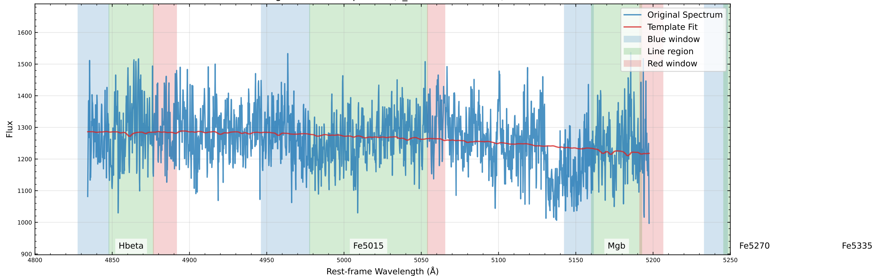
Original Data Comparison (v_star=-1959.5 km/s)
