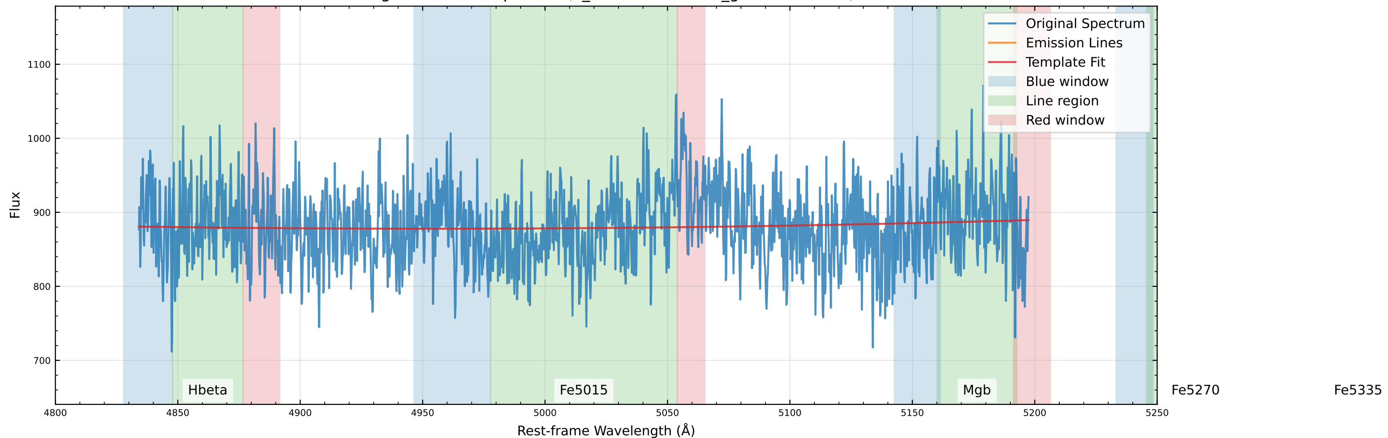
Original Data Comparison (v_star=0.0 km/s, v_gas=31.5 km/s)
