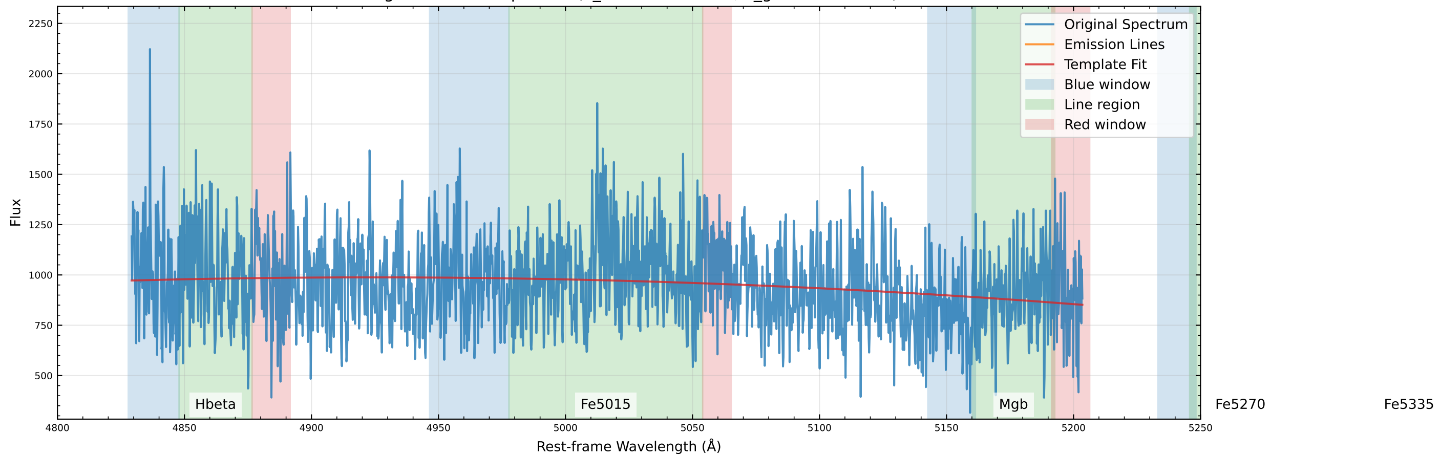
Original Data Comparison (v_star=-30.8 km/s, v_gas=-55.7 km/s)
