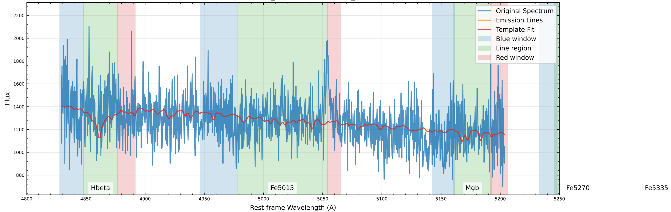
Original Data Comparison (v_star=-472.2 km/s, v_gas=-565.6 km/s)
