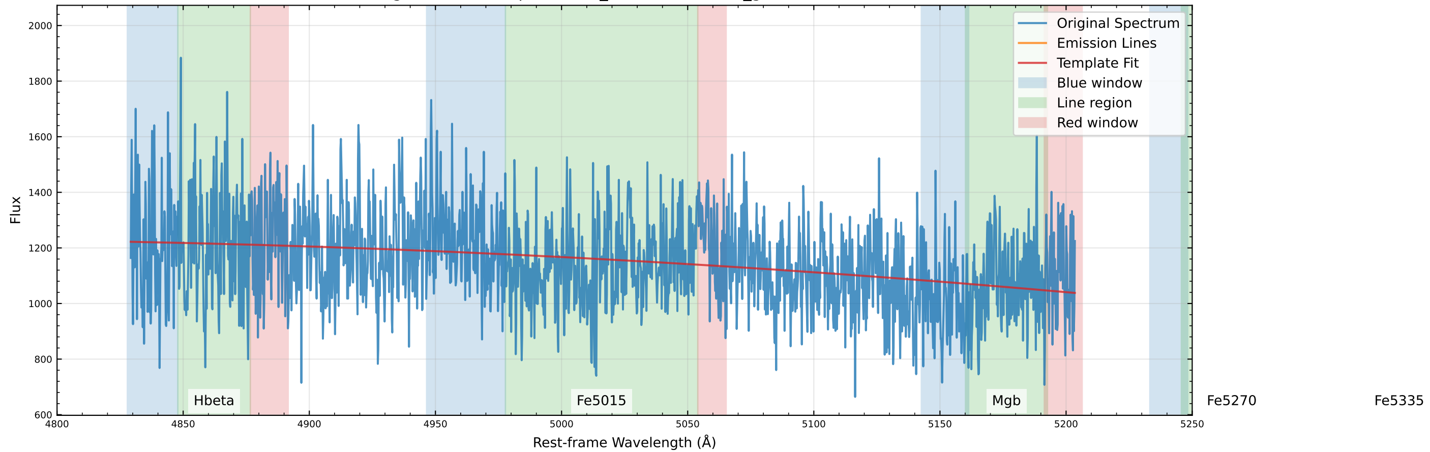
Original Data Comparison ( v_{\text{star}}=0.0 km/s, v_{\text{gas}}=79.3 km/s)
