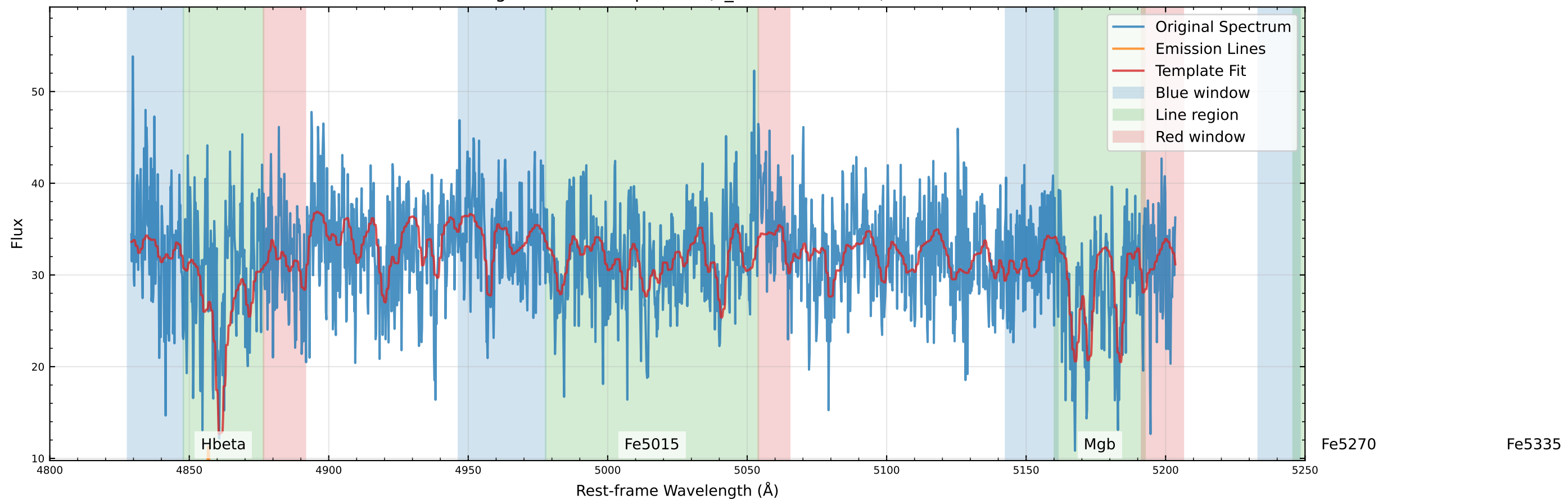
Original Data Comparison (v_star=-47.8 km/s)
