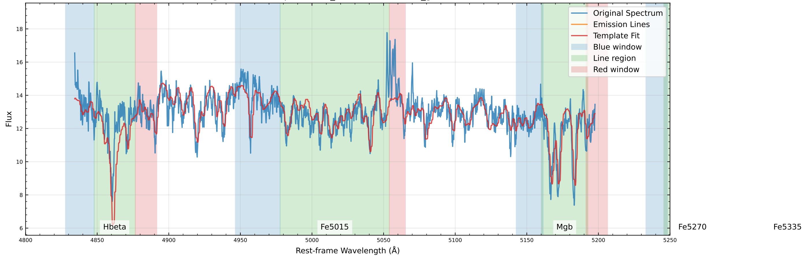
Original Data Comparison (v_star=-42.2 km/s, v_gas=-3.6 km/s)
