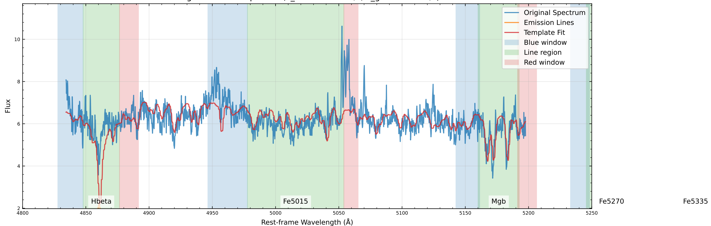
Original Data Comparison (v_star=-40.4 km/s, v_gas=35.3 km/s)
