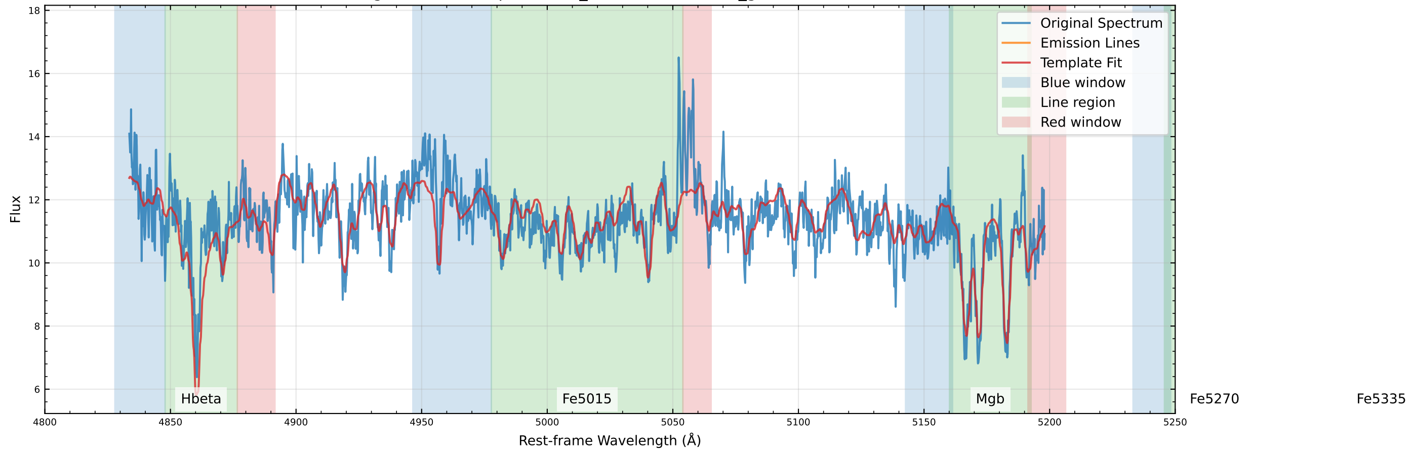
Original Data Comparison (v_star=-42.8 km/s, v_gas=-4.4 km/s)
