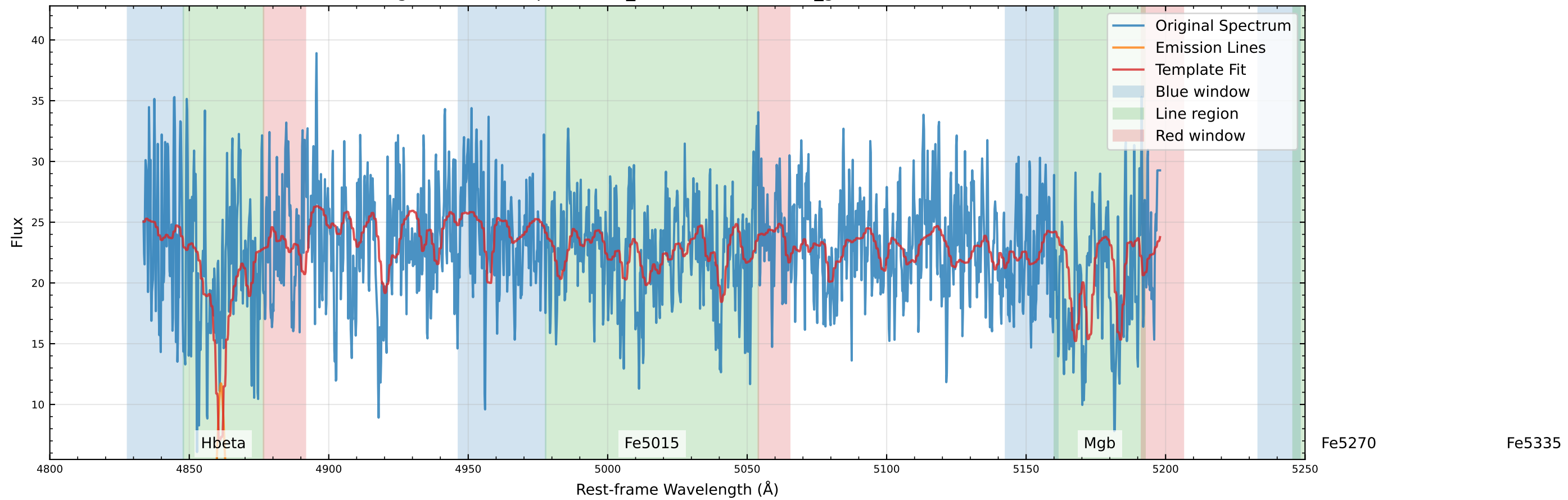
Original Data Comparison (v_star=-111.6 km/s, v_gas=-120.1 km/s)
