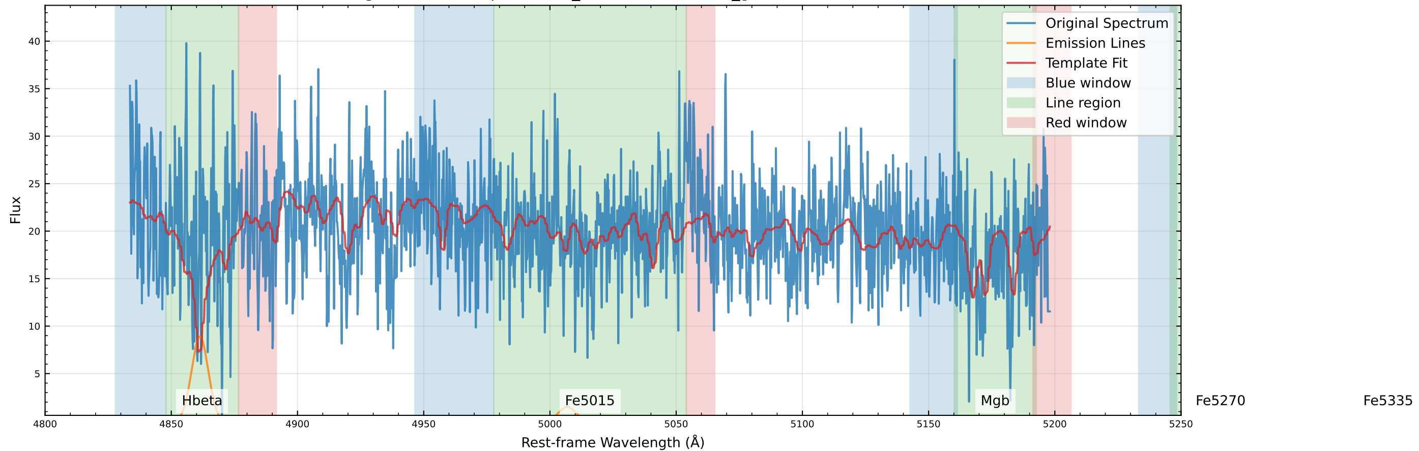
Original Data Comparison (v_star=-90.4 km/s, v_gas=-140.9 km/s)
