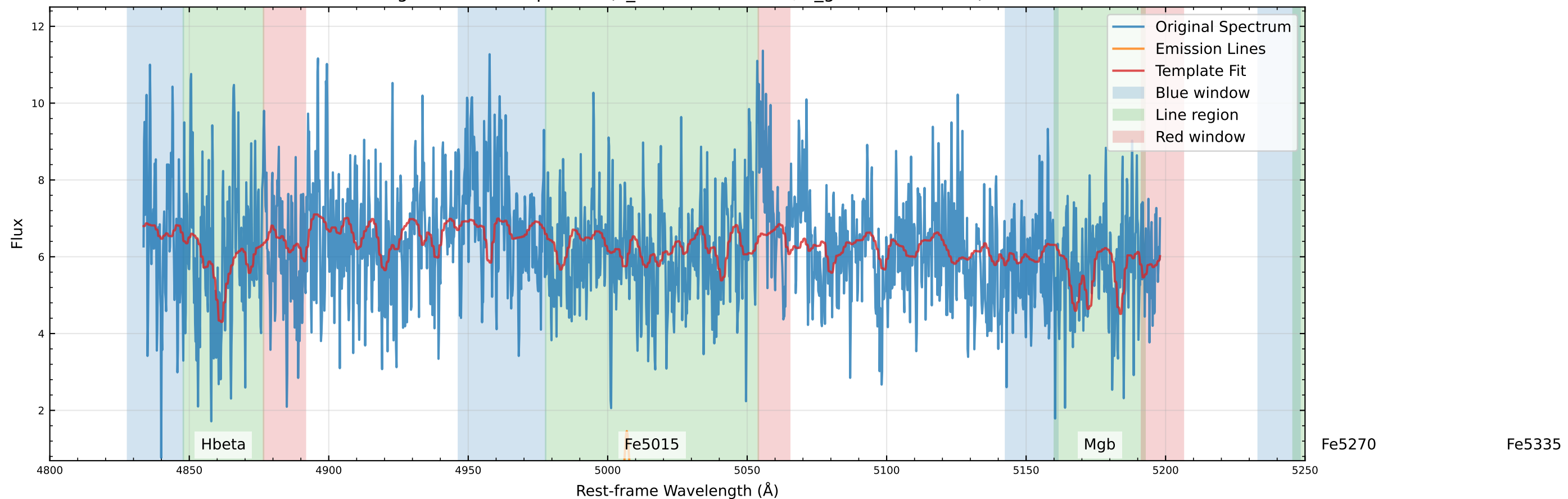
Original Data Comparison (v_star=-118.9 km/s, v_gas=-127.9 km/s)
