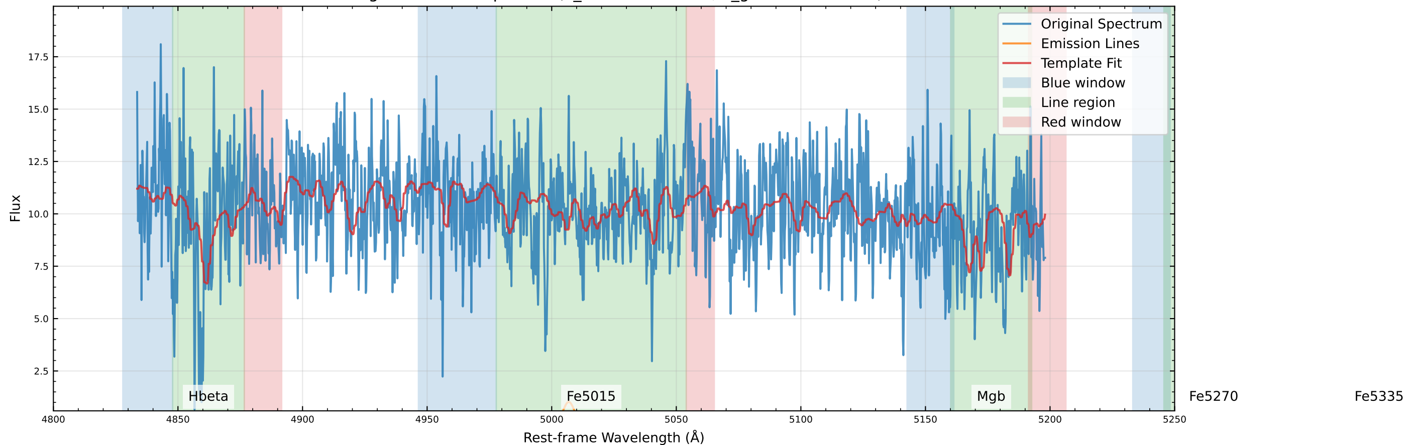
Original Data Comparison (v_star=-98.6 km/s, v_gas=-160.4 km/s)
