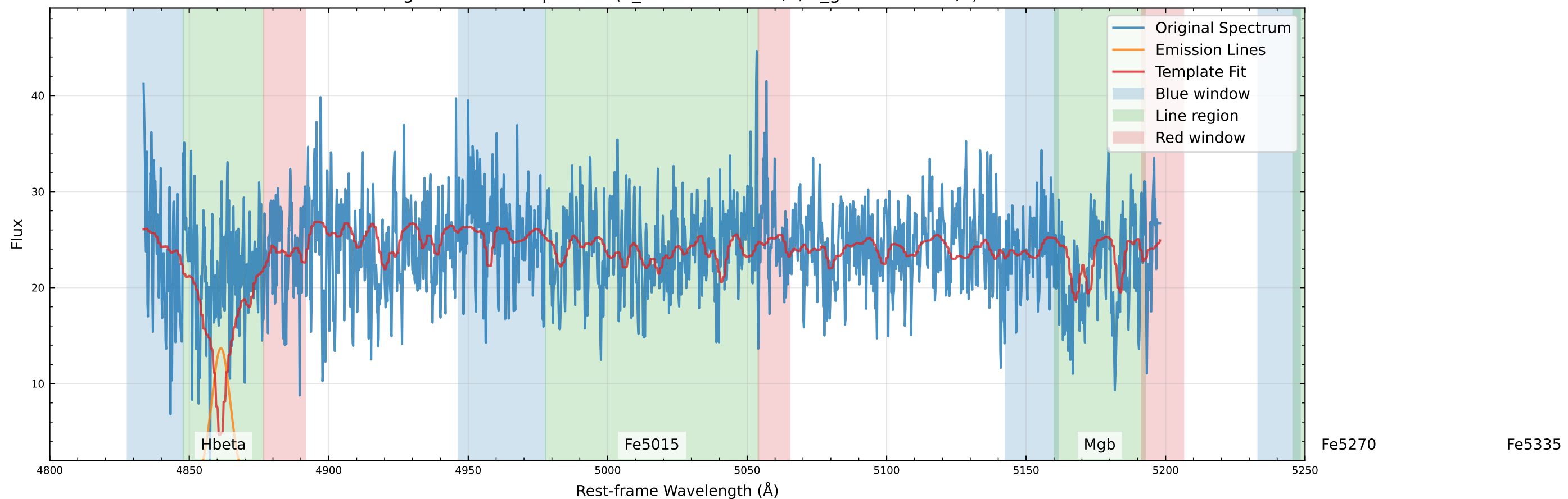
Original Data Comparison (v_star=-113.9 km/s, v_gas=-68.6 km/s)
