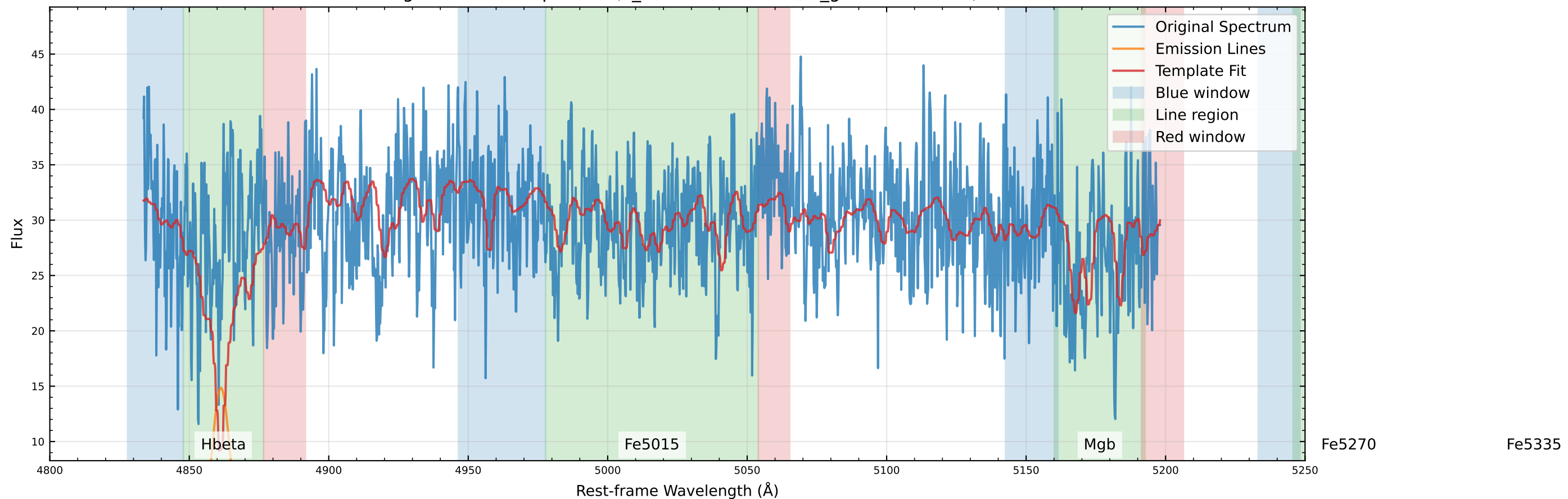
Original Data Comparison (v_star=-102.2 km/s, v_gas=-39.2 km/s)
