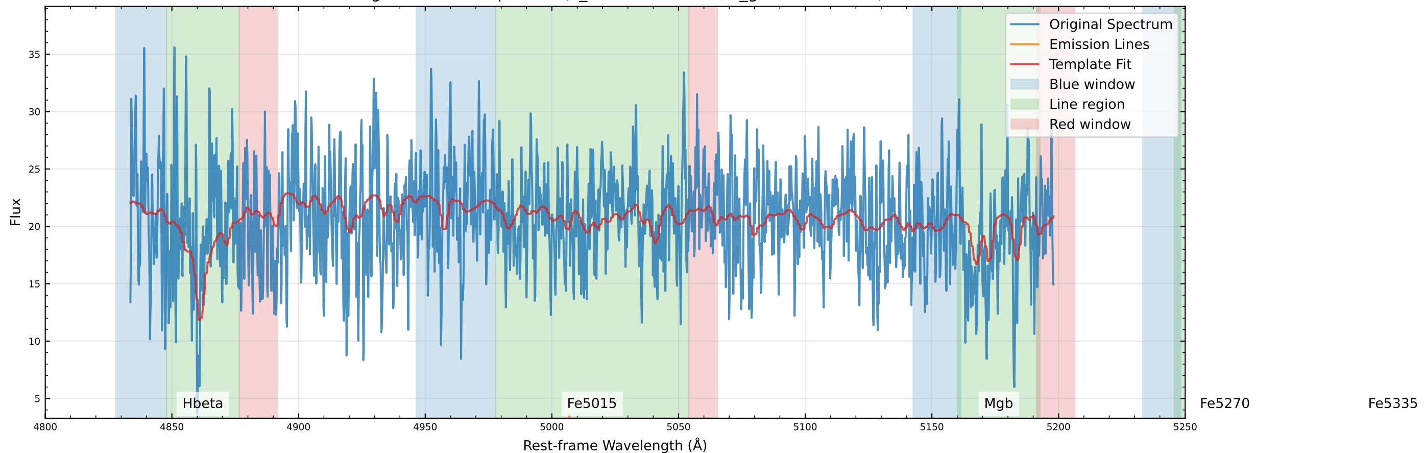
Original Data Comparison ( v_{\text{star}}=-32.6 km/s, v_{\text{gas}}=-40.2 km/s)
