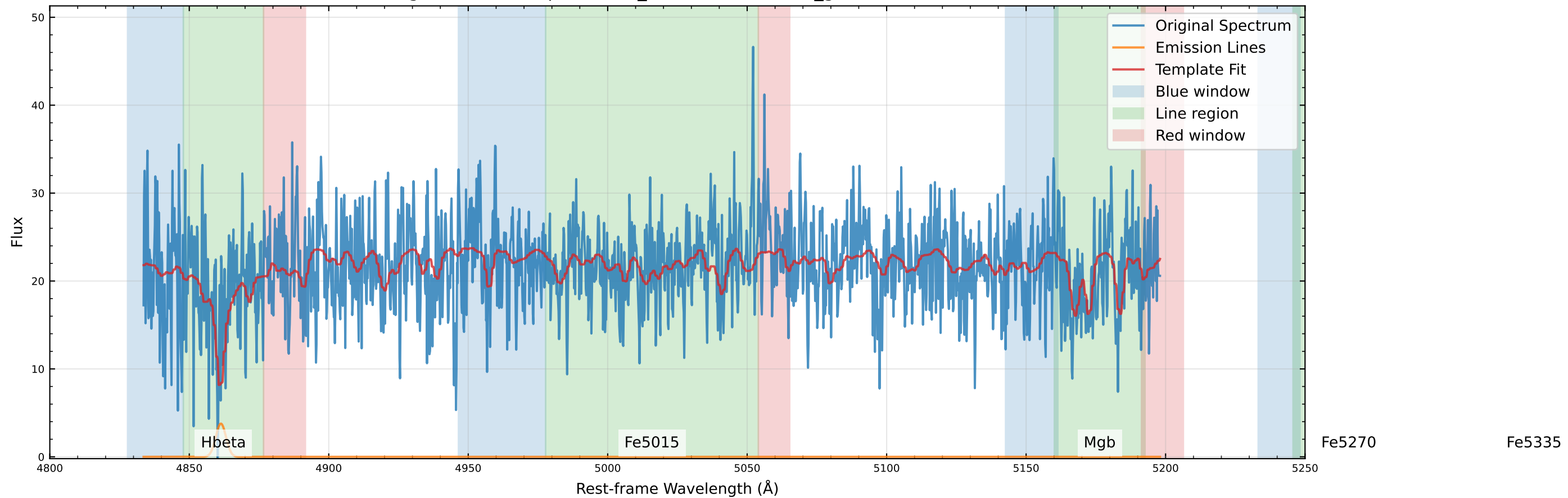
Original Data Comparison (v_star=-40.3 km/s, v_gas=-36.9 km/s)
