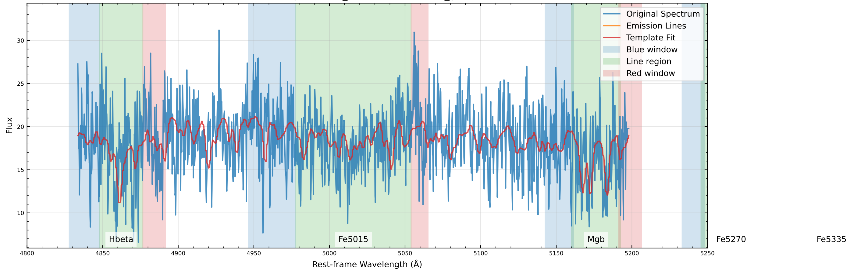
Original Data Comparison (v_star=-120.8 km/s, v_gas=-22.1 km/s)
