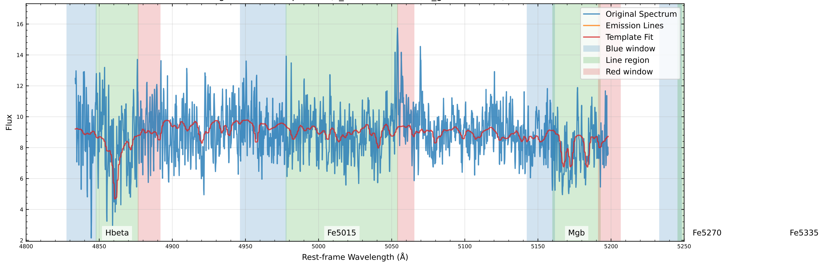
Original Data Comparison (v_star=-51.6 km/s, v_gas=2.7 km/s)
