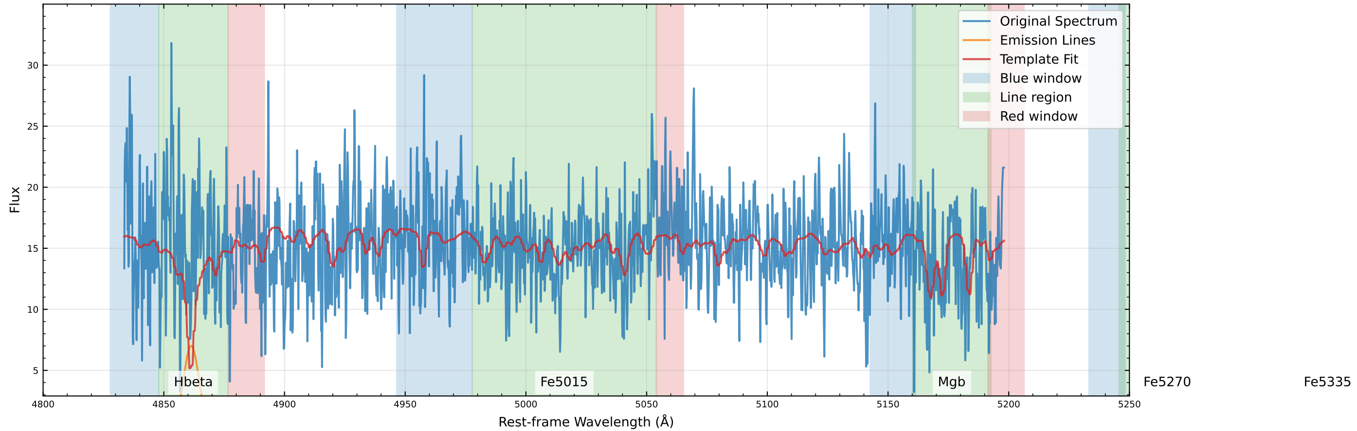
Original Data Comparison ( v_{\text{star}}=-45.4 km/s, v_{\text{gas}}=-13.0 km/s)
