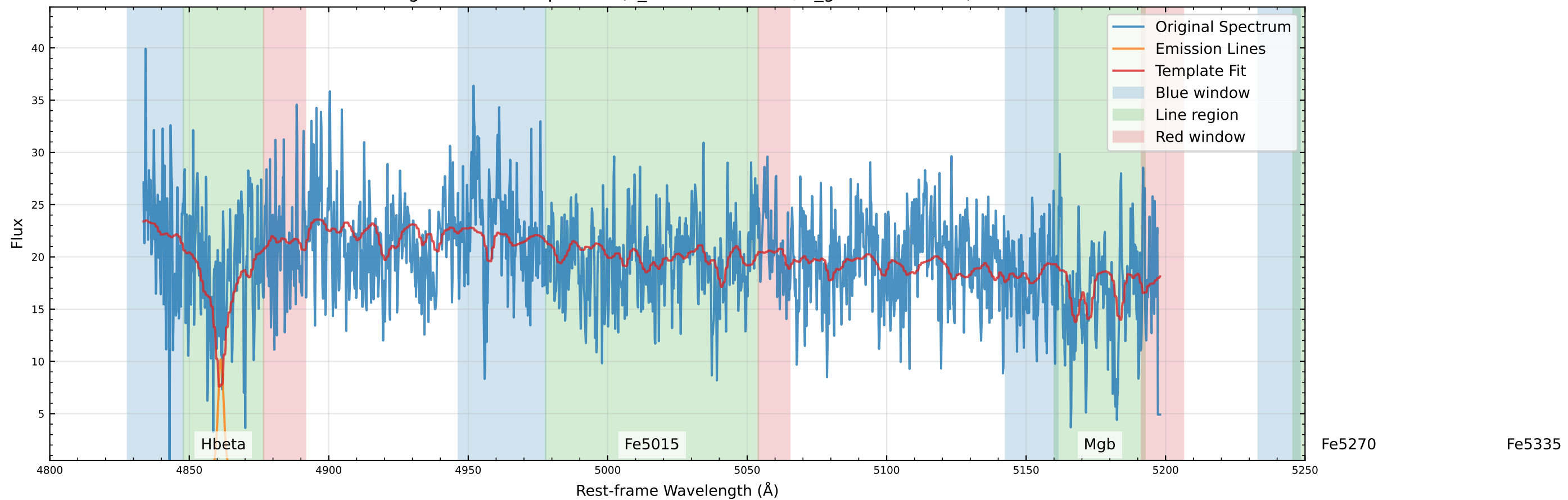
Original Data Comparison (v_star=-96.7 km/s, v_gas=-94.2 km/s)
