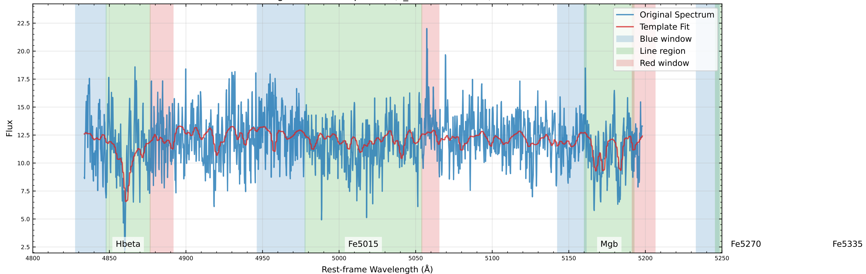
Original Data Comparison (v_star=-45.7 km/s)
