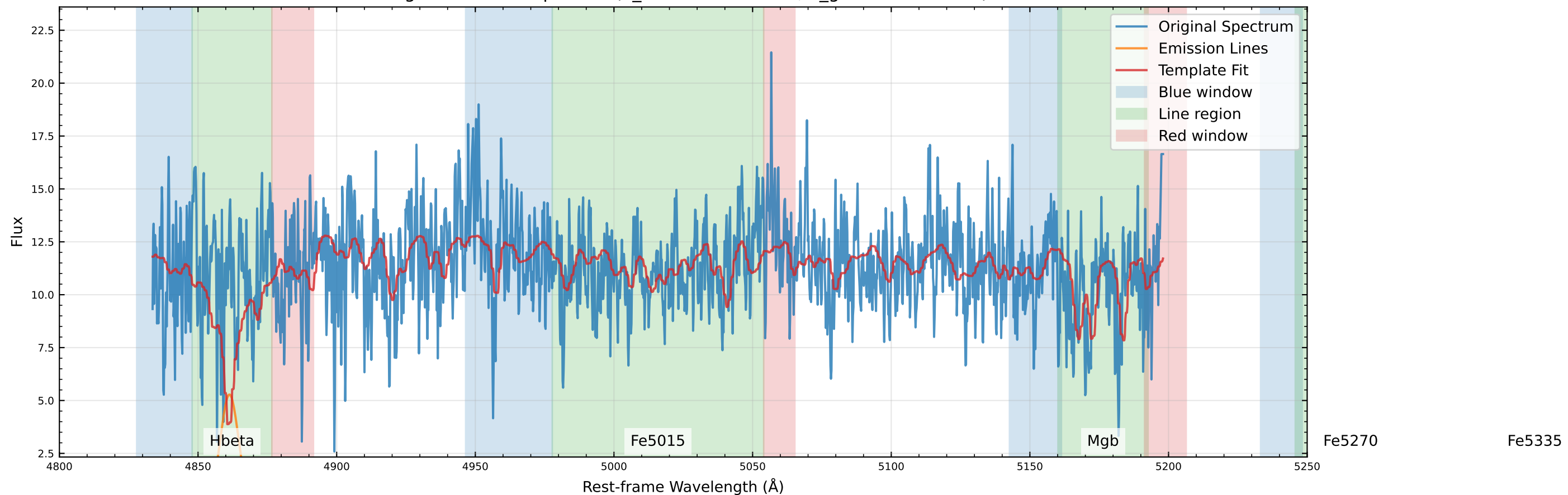
Original Data Comparison (v_star=-101.5 km/s, v_gas=-106.6 km/s)
