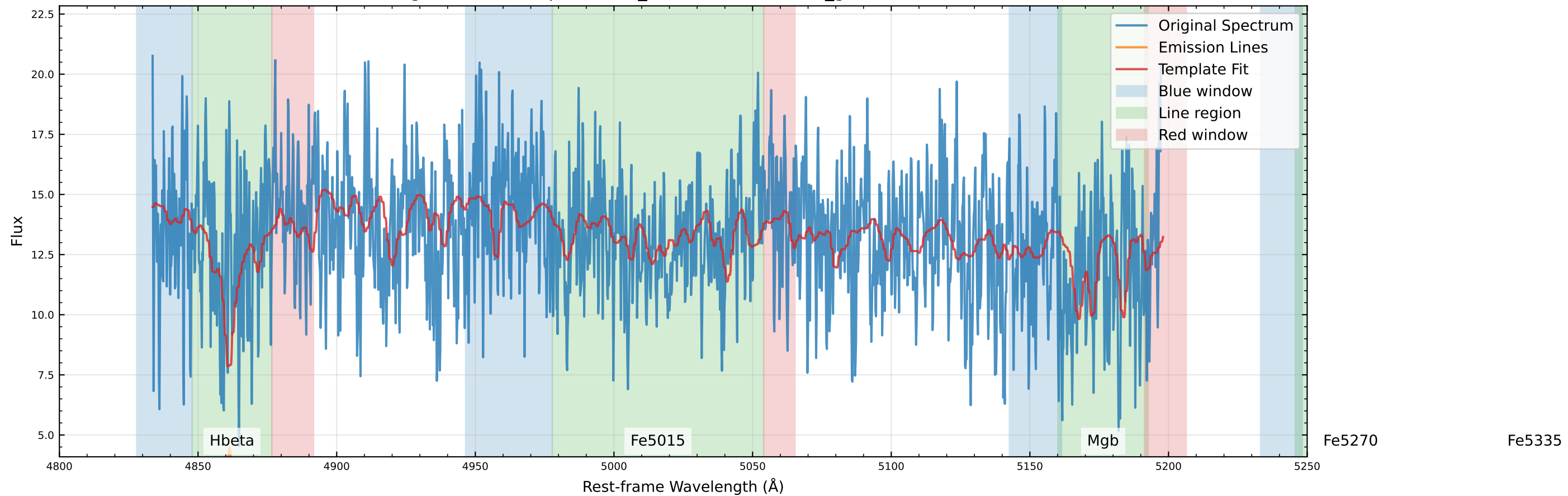
Original Data Comparison ( v_{\text{star}}=-140.2 km/s, v_{\text{gas}}=-42.2 km/s)
