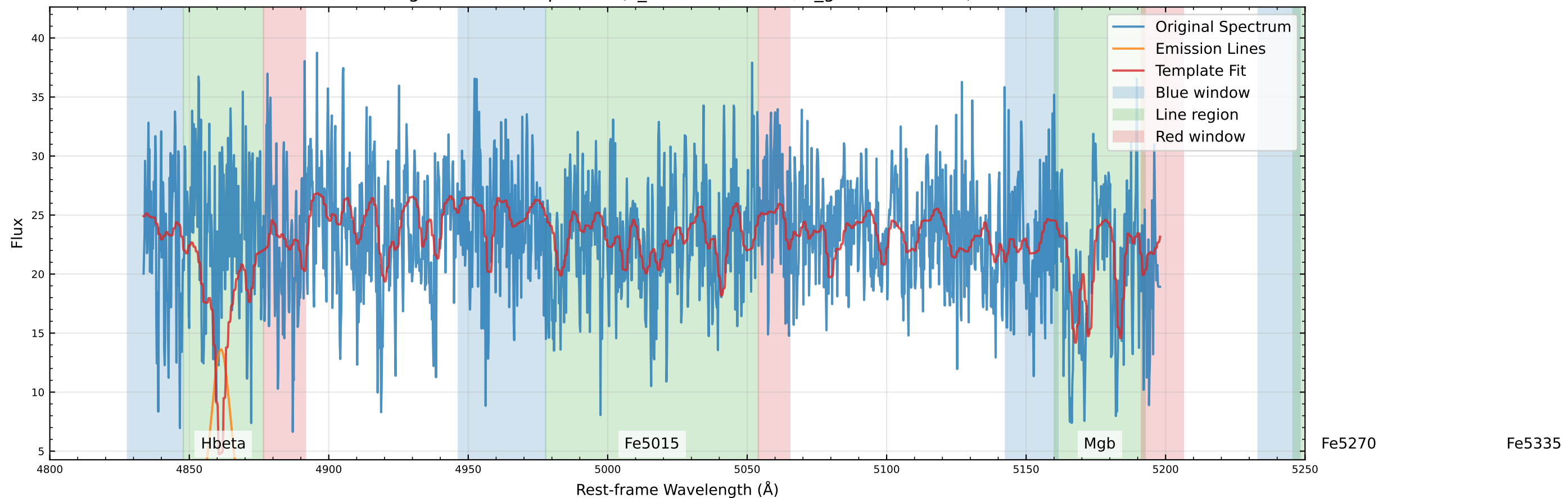
Original Data Comparison (v_star=-82.5 km/s, v_gas=-44.8 km/s)
