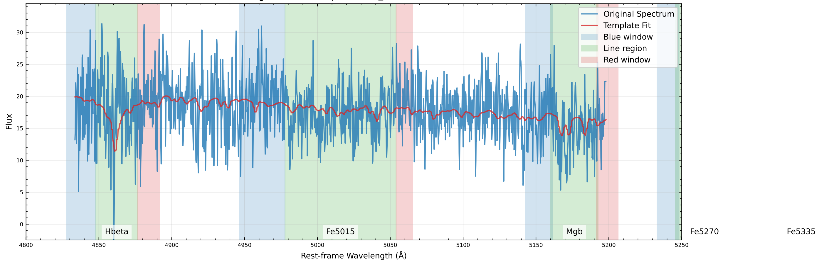
Original Data Comparison (v_star=-44.1 km/s)
