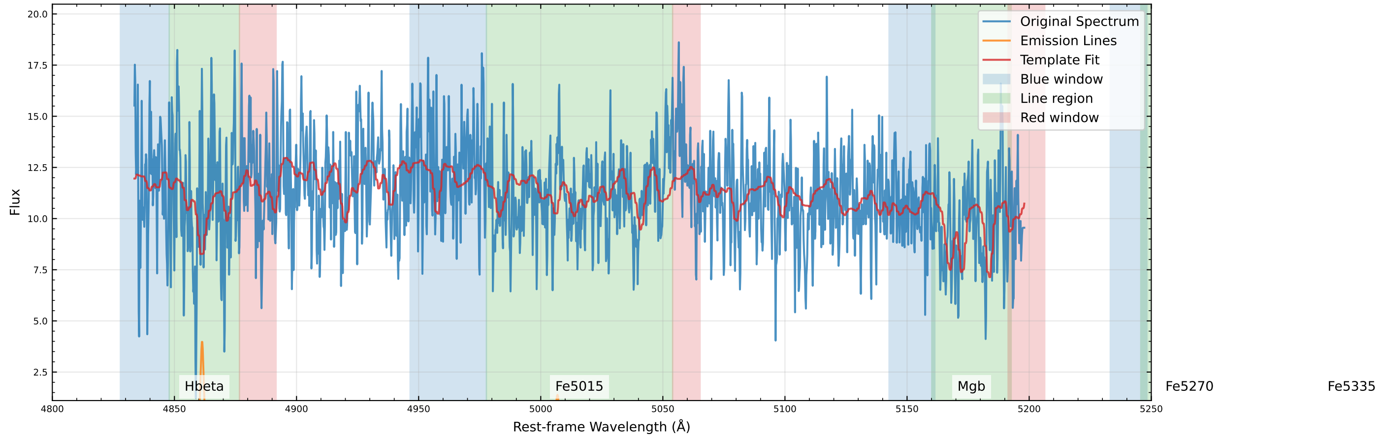
Original Data Comparison (v_star=-94.6 km/s, v_gas=-18.9 km/s)
