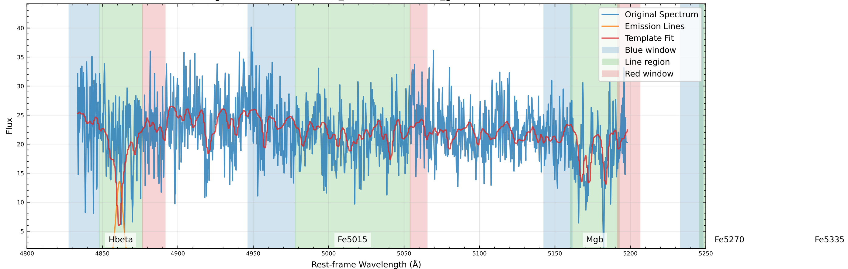
Original Data Comparison (v_star=-103.0 km/s, v_gas=-124.4 km/s)
