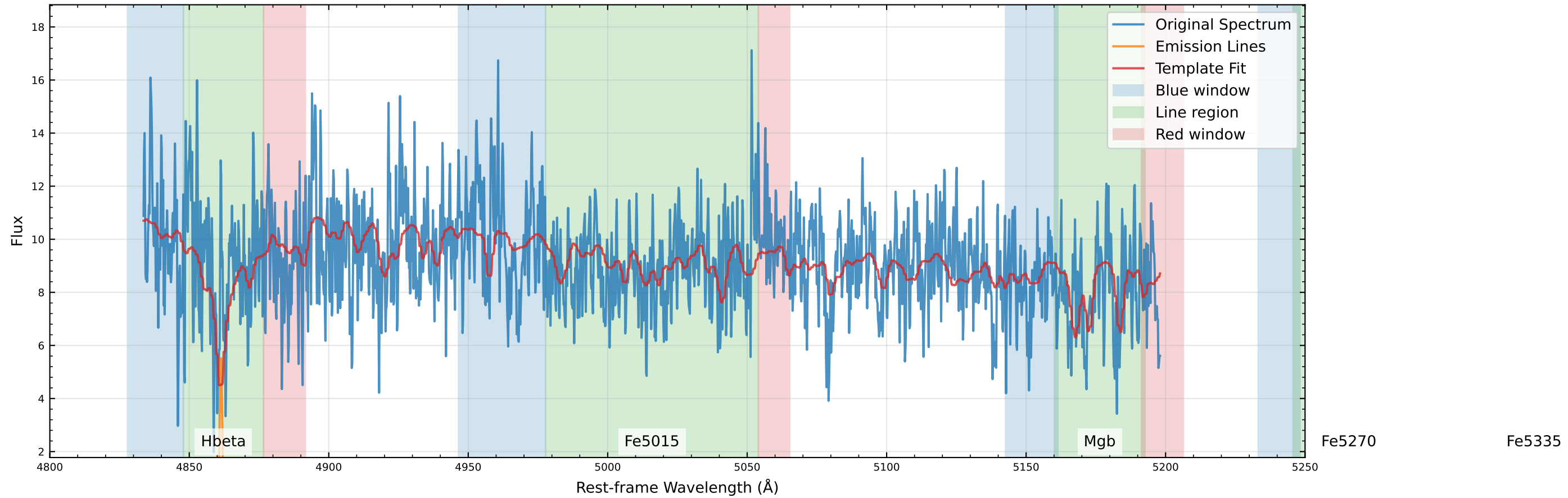
Original Data Comparison (v_star=-75.9 km/s, v_gas=2.6 km/s)
