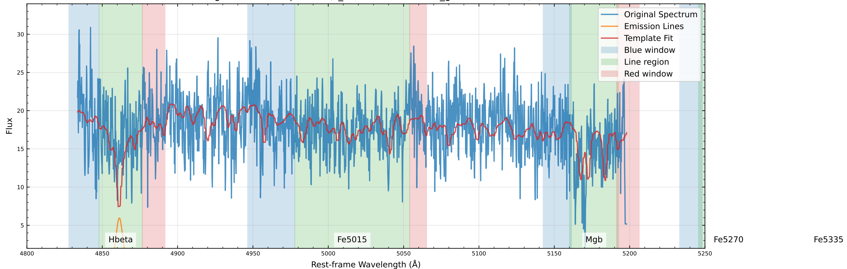
Original Data Comparison (v_star=-138.6 km/s, v_gas=-178.7 km/s)
