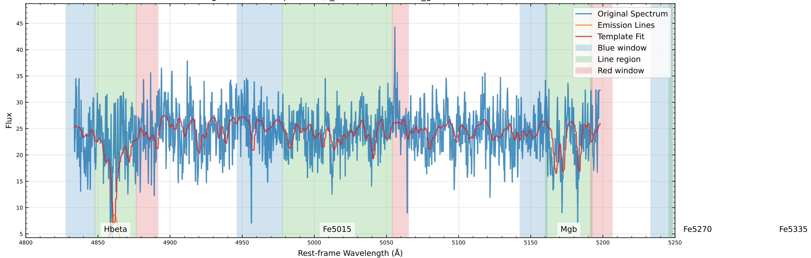
Original Data Comparison (v_star=-93.1 km/s, v_gas=-73.1 km/s)
