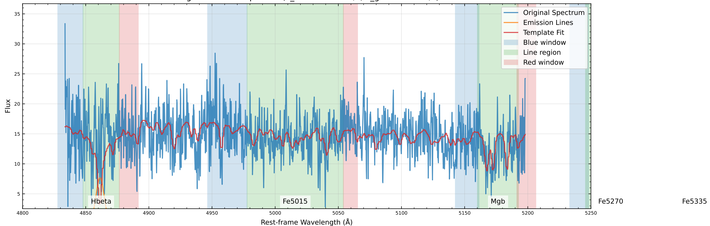
Original Data Comparison (v_star=-33.9 km/s, v_gas=20.7 km/s)
