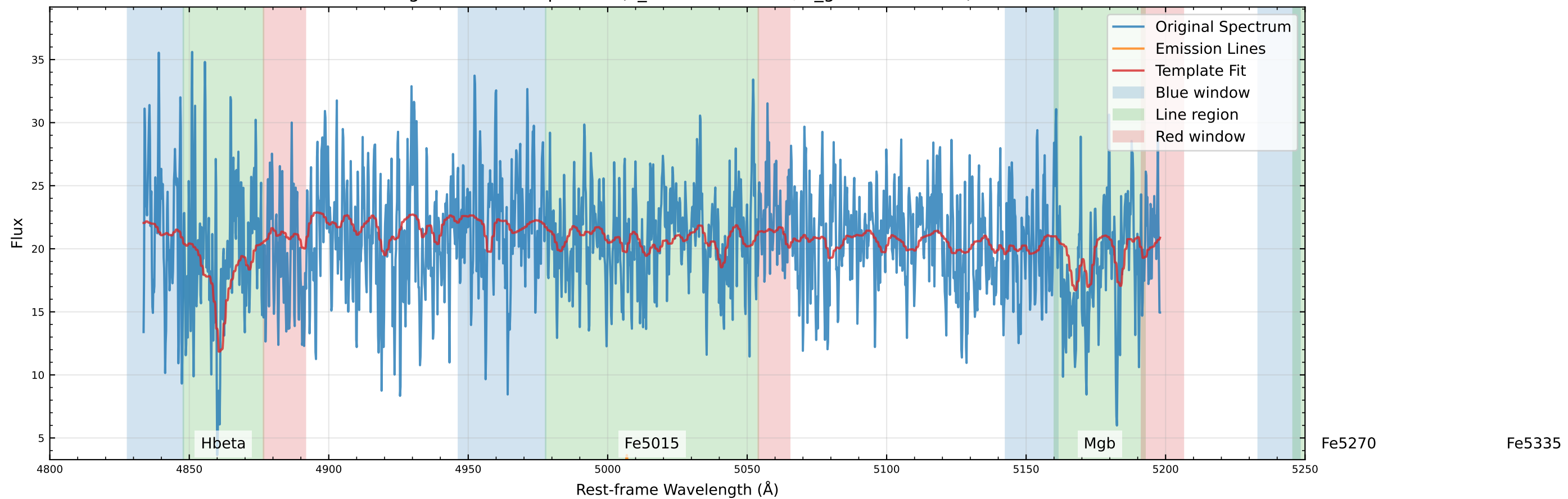
Original Data Comparison (v_star=-32.6 km/s, v_gas=-40.2 km/s)
