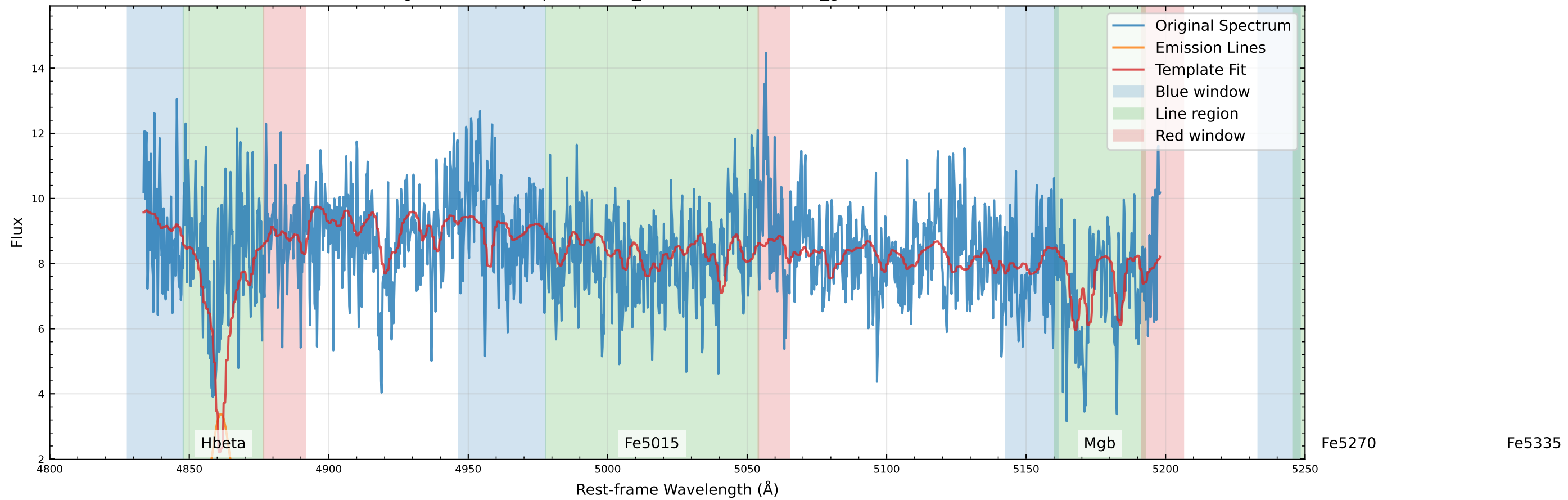
Original Data Comparison (v_star=-107.7 km/s, v_gas=-37.0 km/s)
