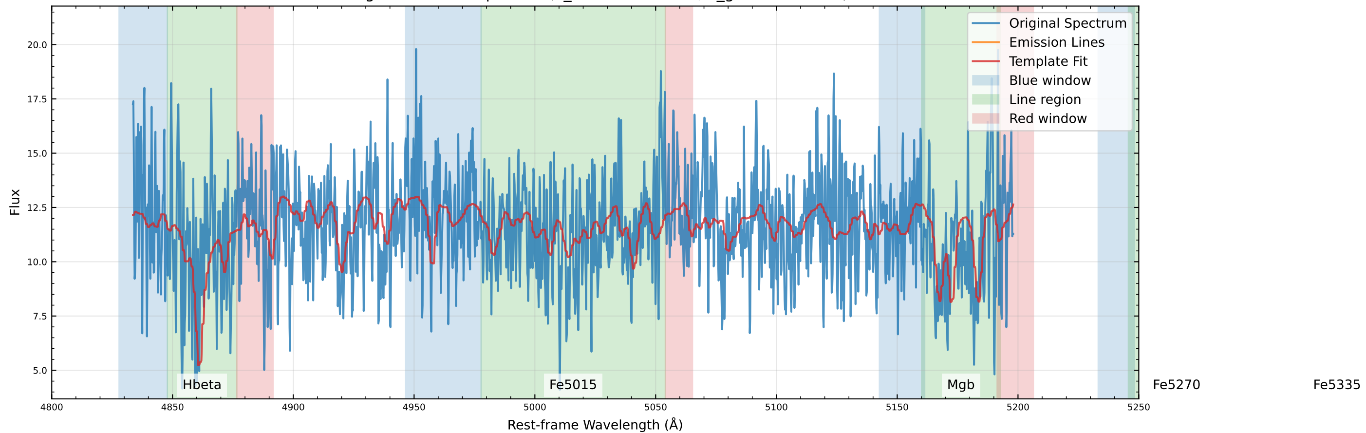
Original Data Comparison (v_star=-74.1 km/s, v_gas=31.4 km/s)
