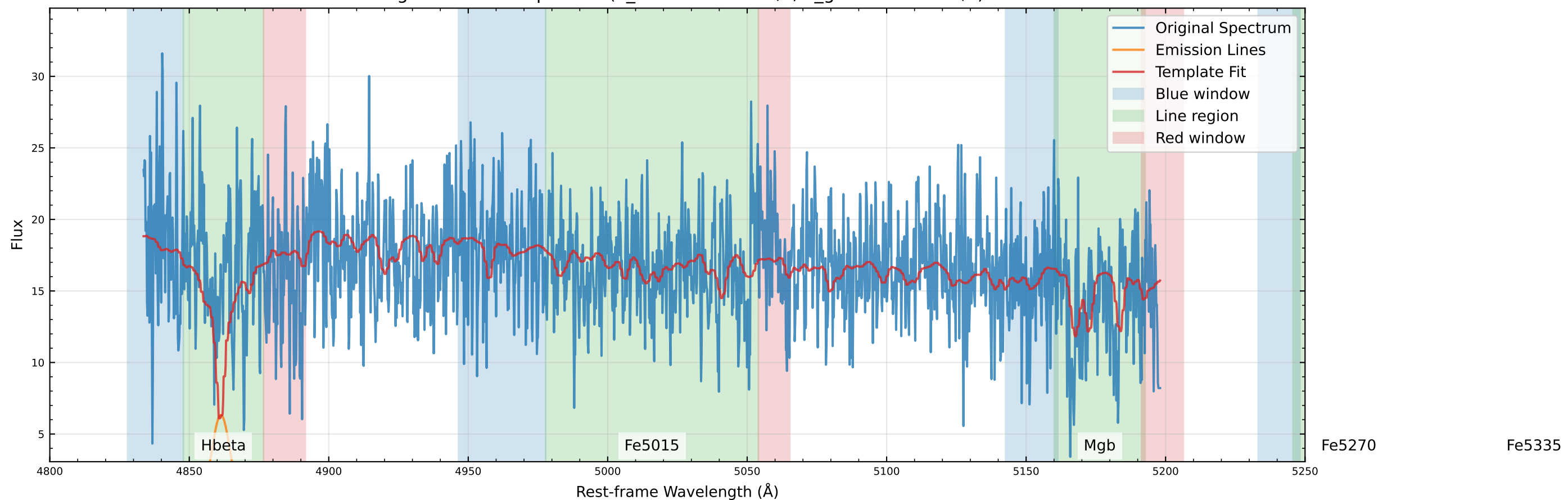
Original Data Comparison (v_star=-104.4 km/s, v_gas=-167.3 km/s)
