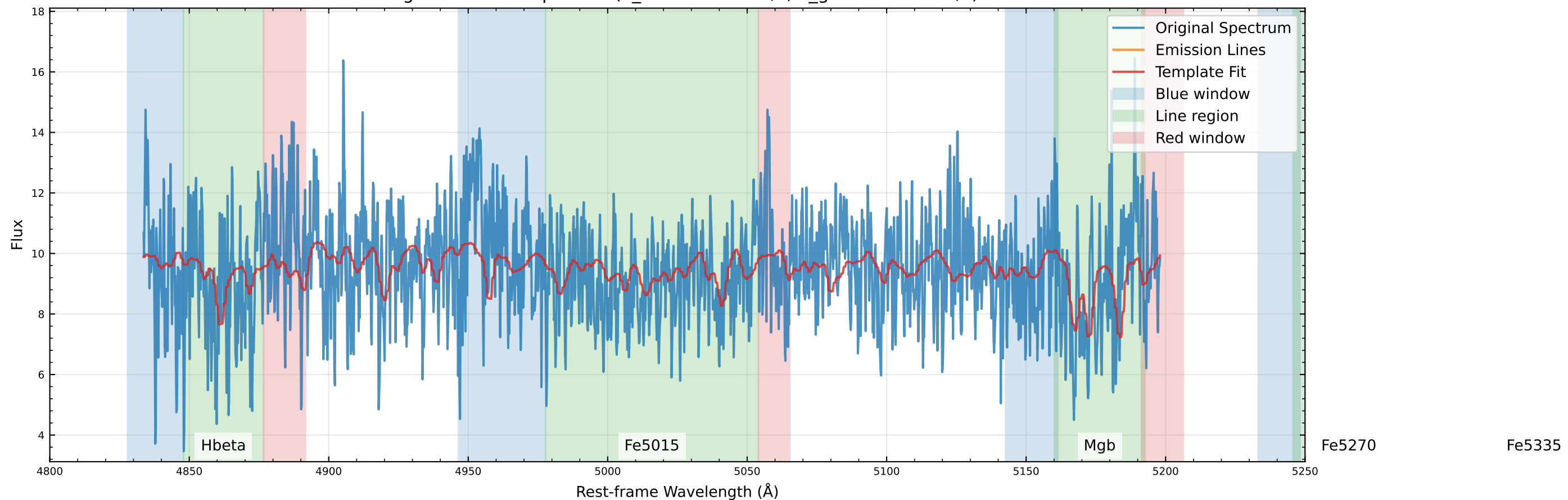
Original Data Comparison (v_star=-78.0 km/s, v_gas=-117.8 km/s)
