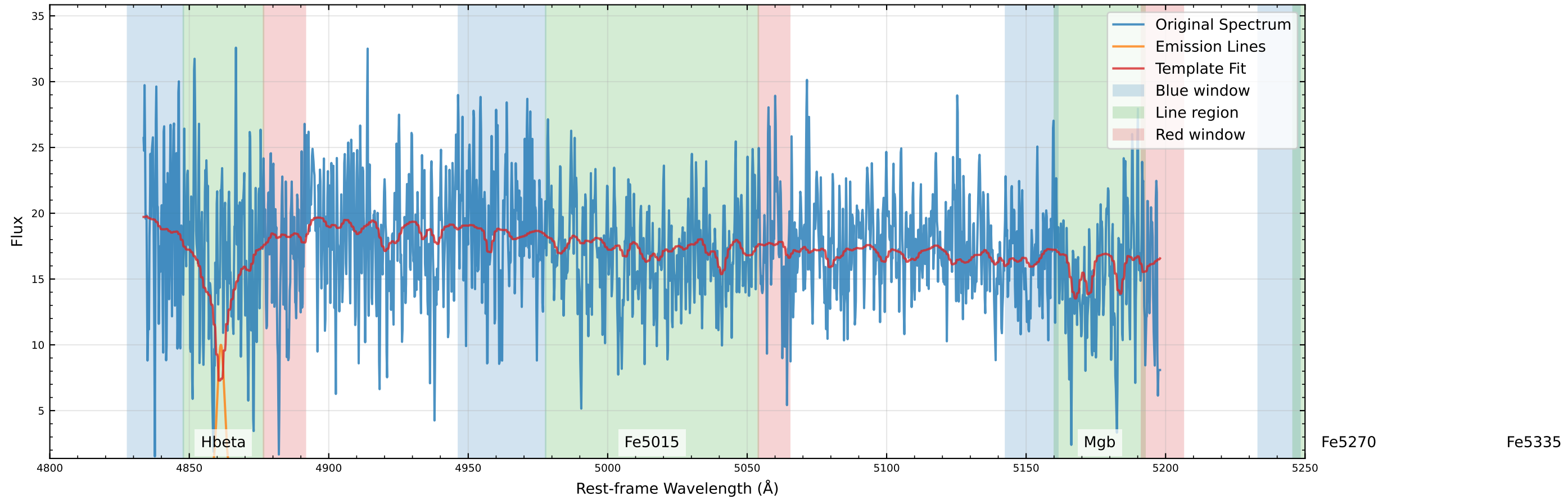
Original Data Comparison (v_star=-78.3 km/s, v_gas=-15.2 km/s)
