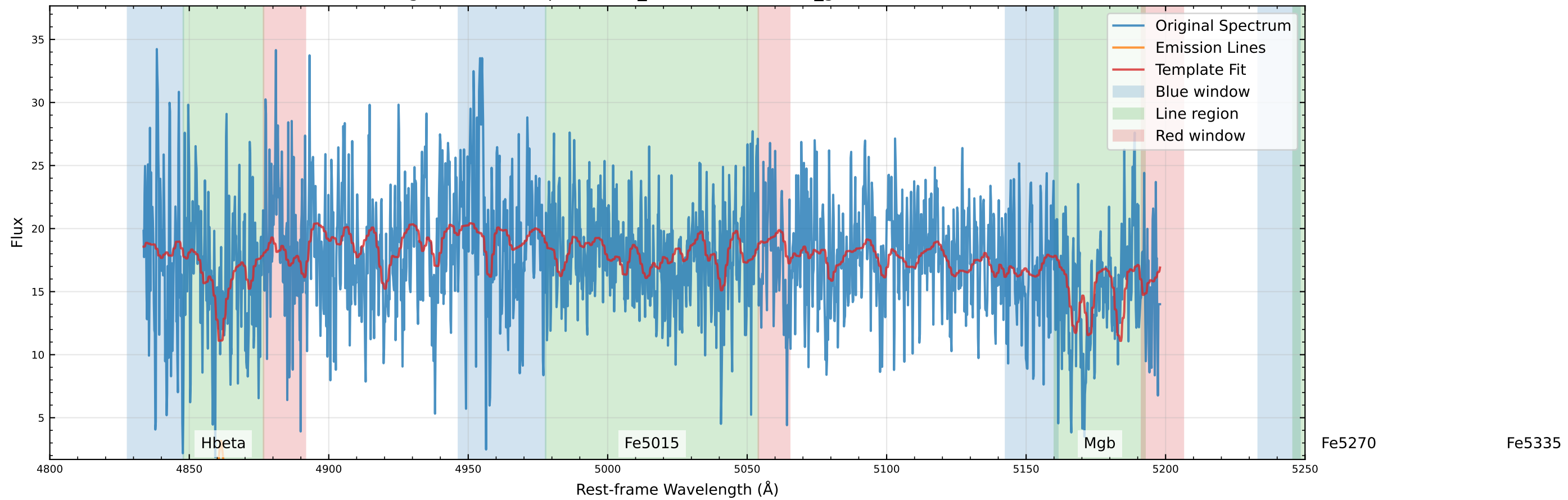
Original Data Comparison (v_star=-65.9 km/s, v_gas=-55.2 km/s)
