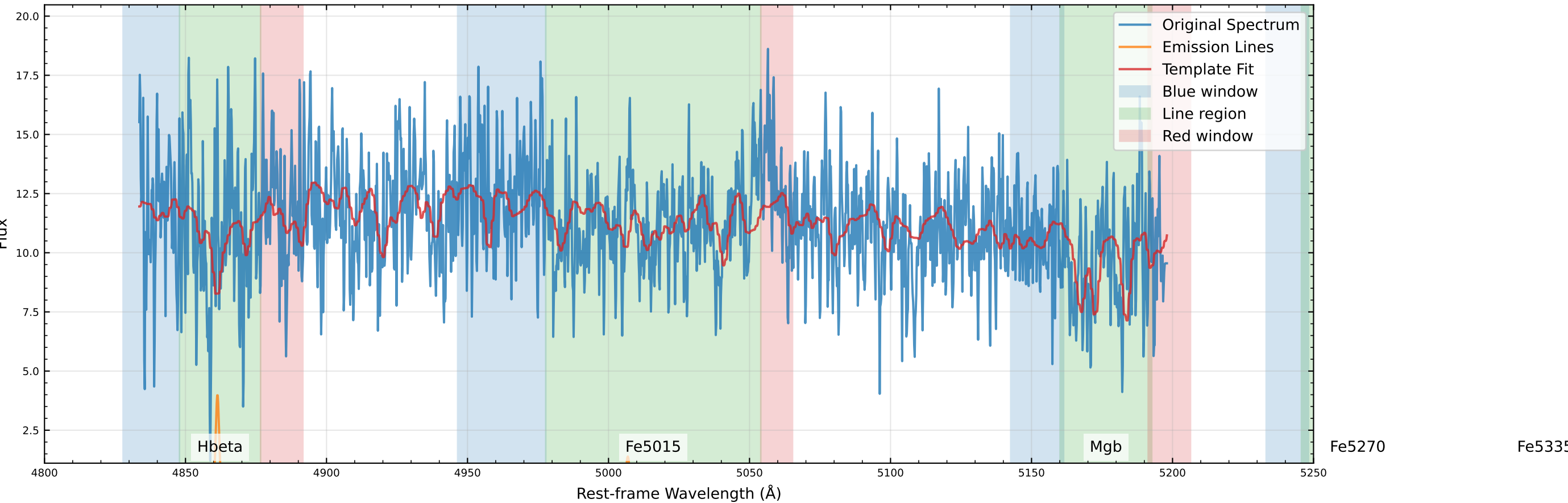
Original Data Comparison (v_star=-94.6 km/s, v_gas=-18.9 km/s)
