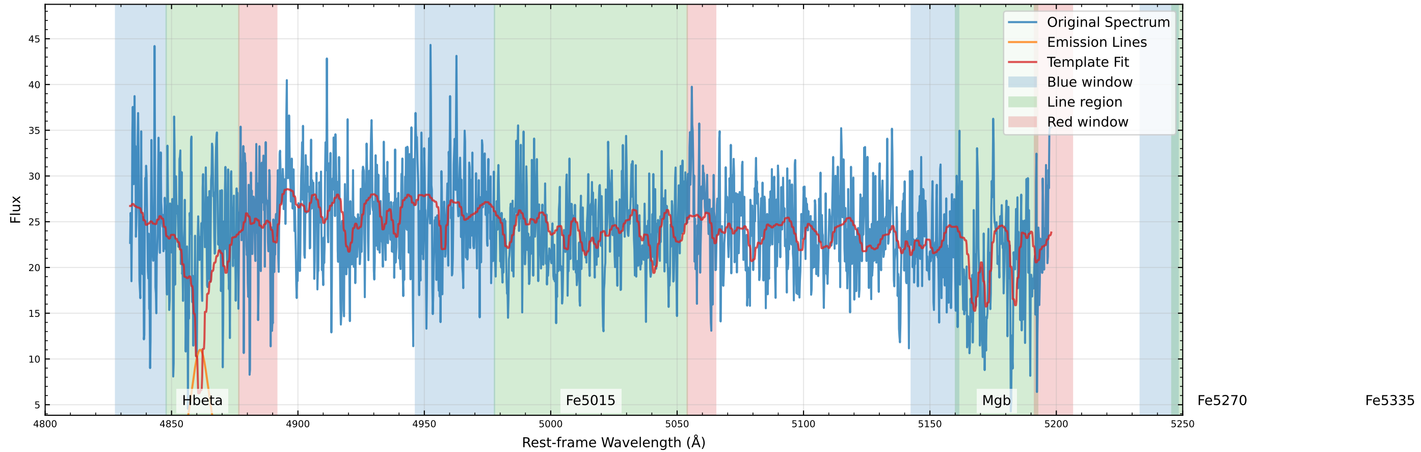
Original Data Comparison (v_star=-84.3 km/s, v_gas=12.6 km/s)
