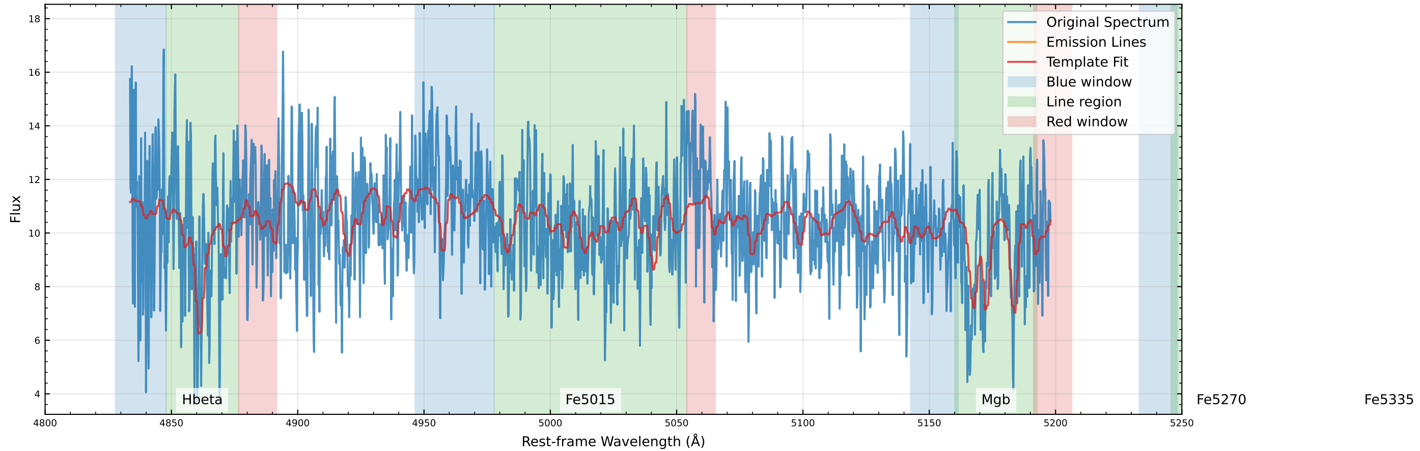
Original Data Comparison (v_star=-52.1 km/s, v_gas=-49.1 km/s)
